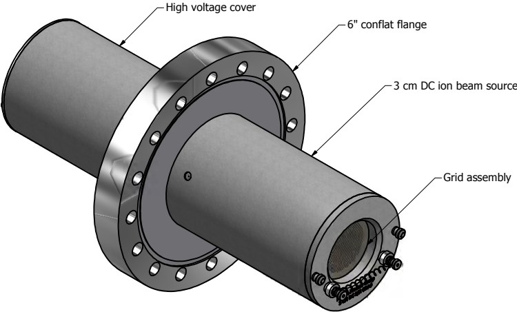
504868A - 6.0" conflat flange mount (with source and grids).
