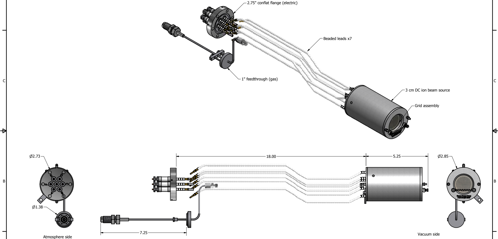
505406A - internal mount with 2.75" CF and 1" o-ring feedthroughs (with source and grids).
