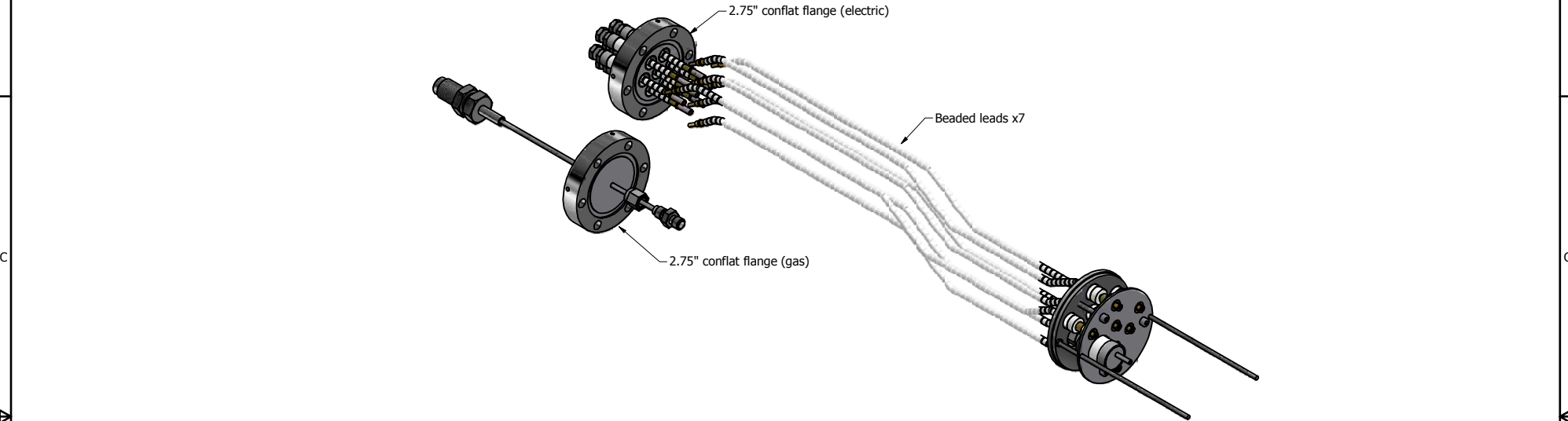
505371A - internal mount with 2.75" CF x2 feedthroughs (with source and grids).
