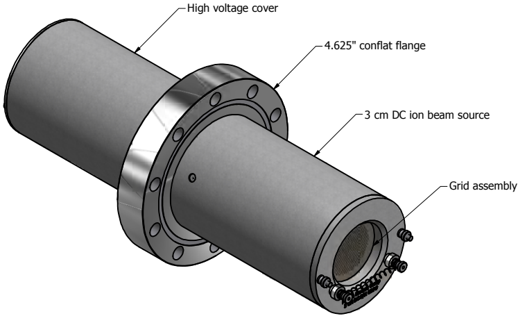
504694A - 4.625" conflat flange mount (with source and grids).
