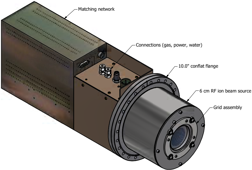
505865A - 10.0" conflat flange mount (with source, grids and matching network)
