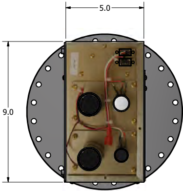
Atmosphere side
