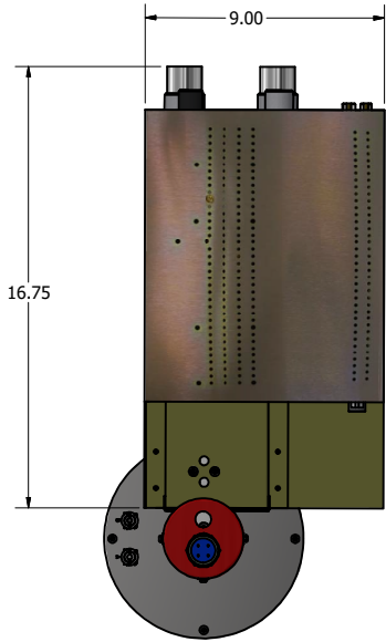
Atmosphere side
