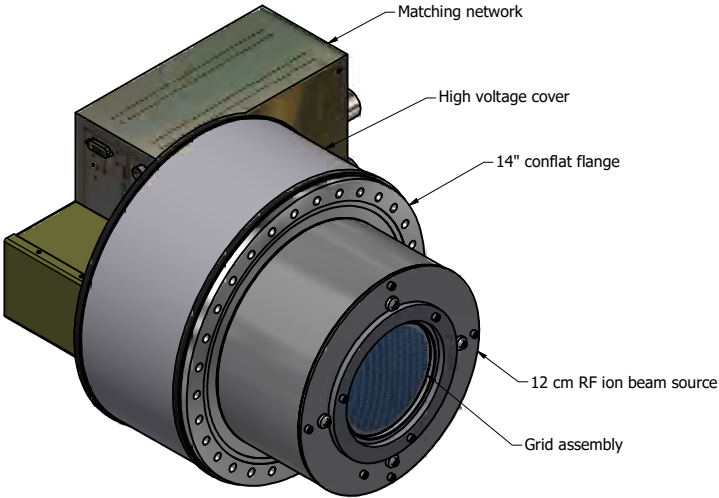
504904A - 14" conflat flange mount (with source, grids and matching network).
