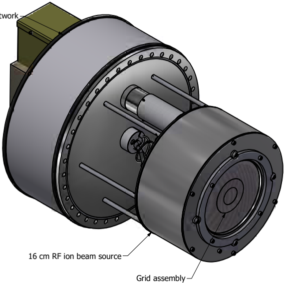
504902A - 16.5 conflat flange extension mount (with source, grids and matching network).
