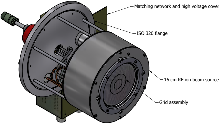
505038A - 320 ISO flange extension mount (with source, grids and matching network).
