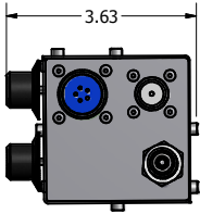
Atmosphere side
