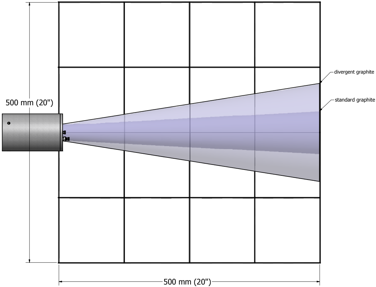
SIDE VIEW
